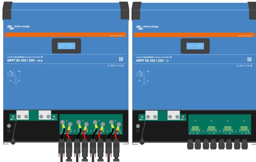
The MC4 connectors are pre-wired whereas the "- Tr" version has screw terminal blocks, PV wires pass through cable glands at the bottom of the unit.
